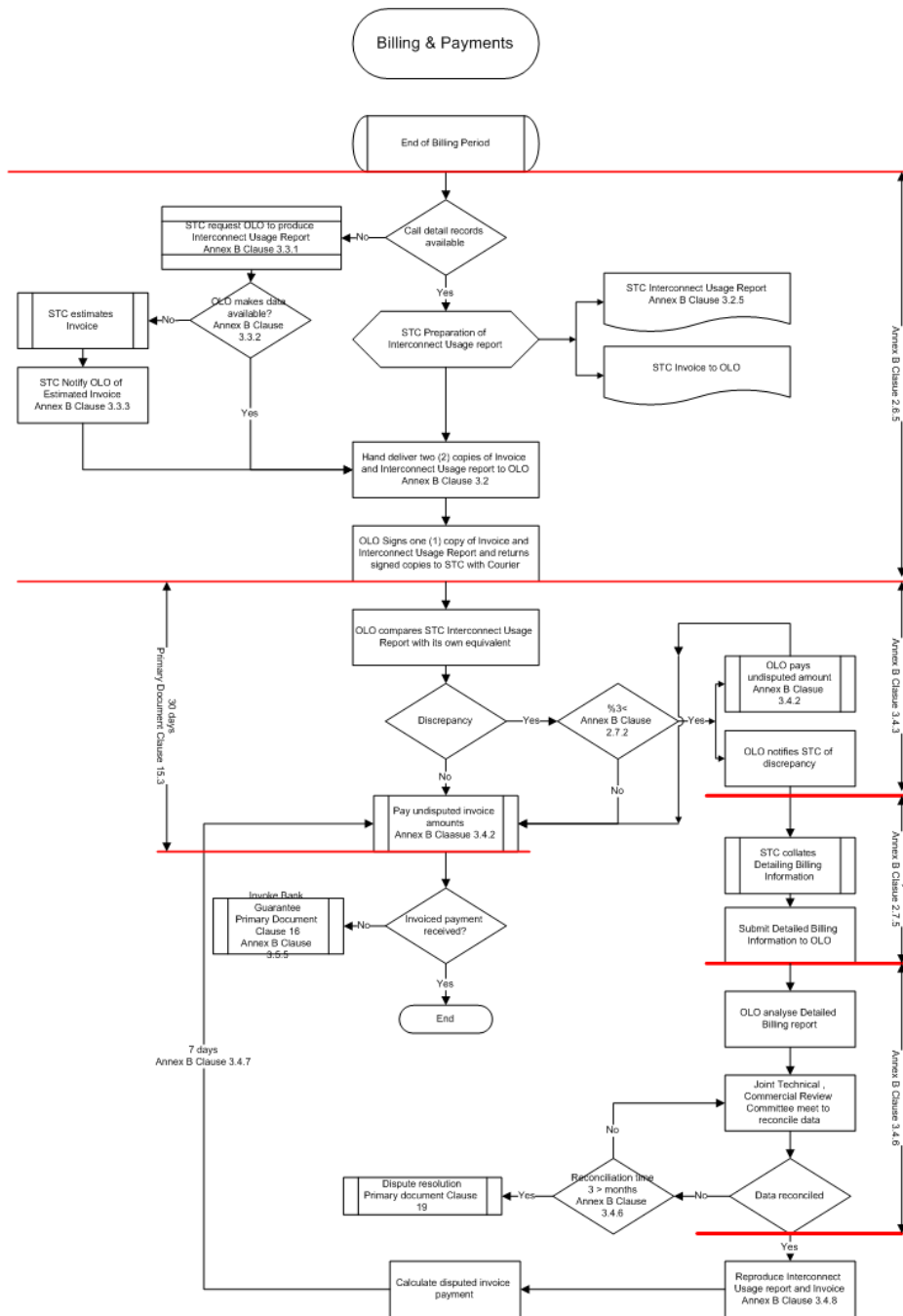
Invoicing Flow Diagram
